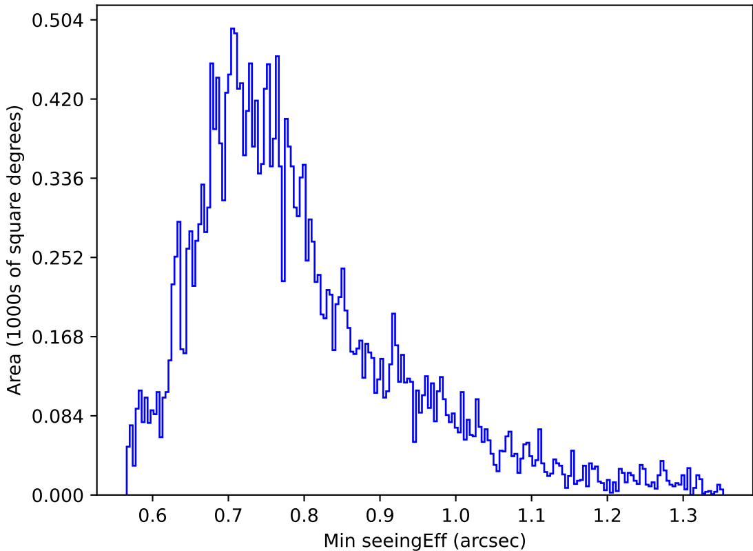
too_elab_r256_d3_ugrizy_v3.4_10yrs Yr 1 g band: Min seeingEff
