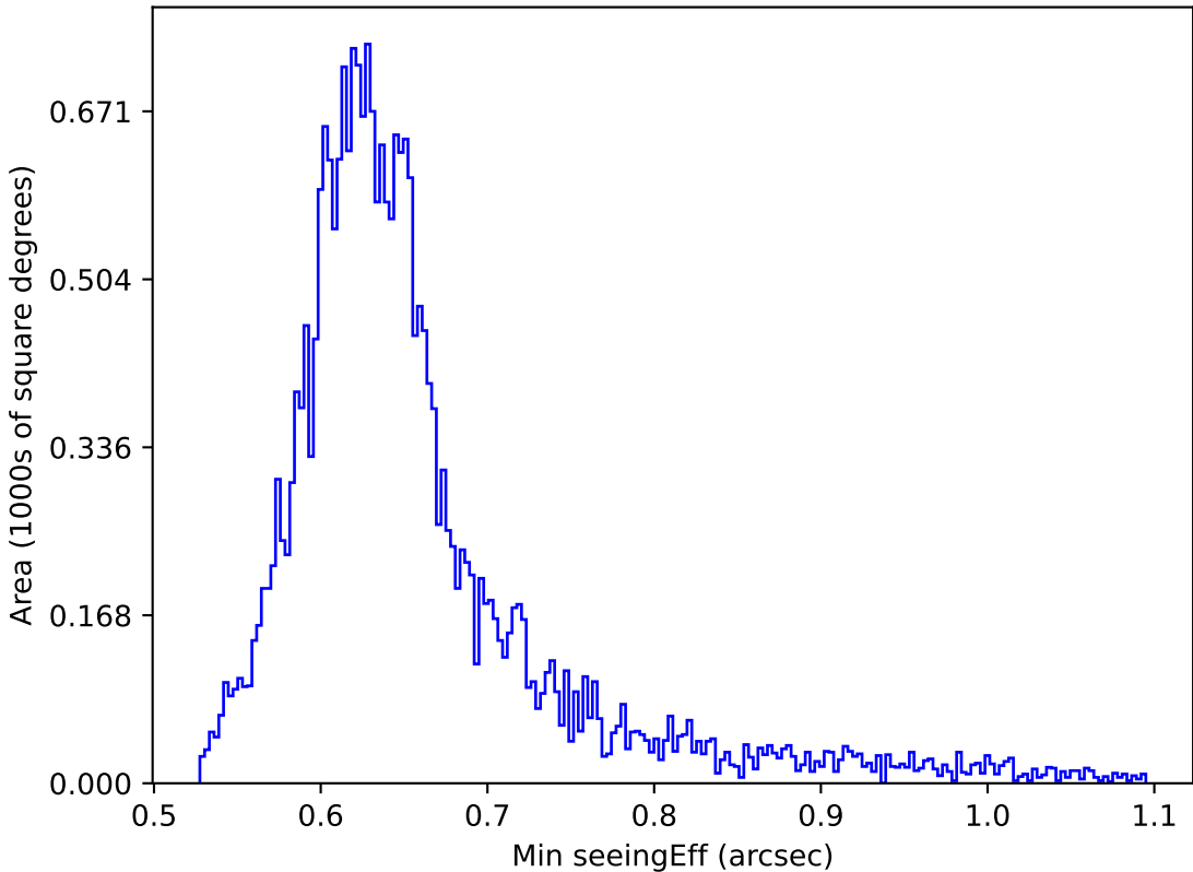
too_elab_r256_d3_ugrizy_v3.4_10yrs Yr 1 all bands: Min seeingEff
