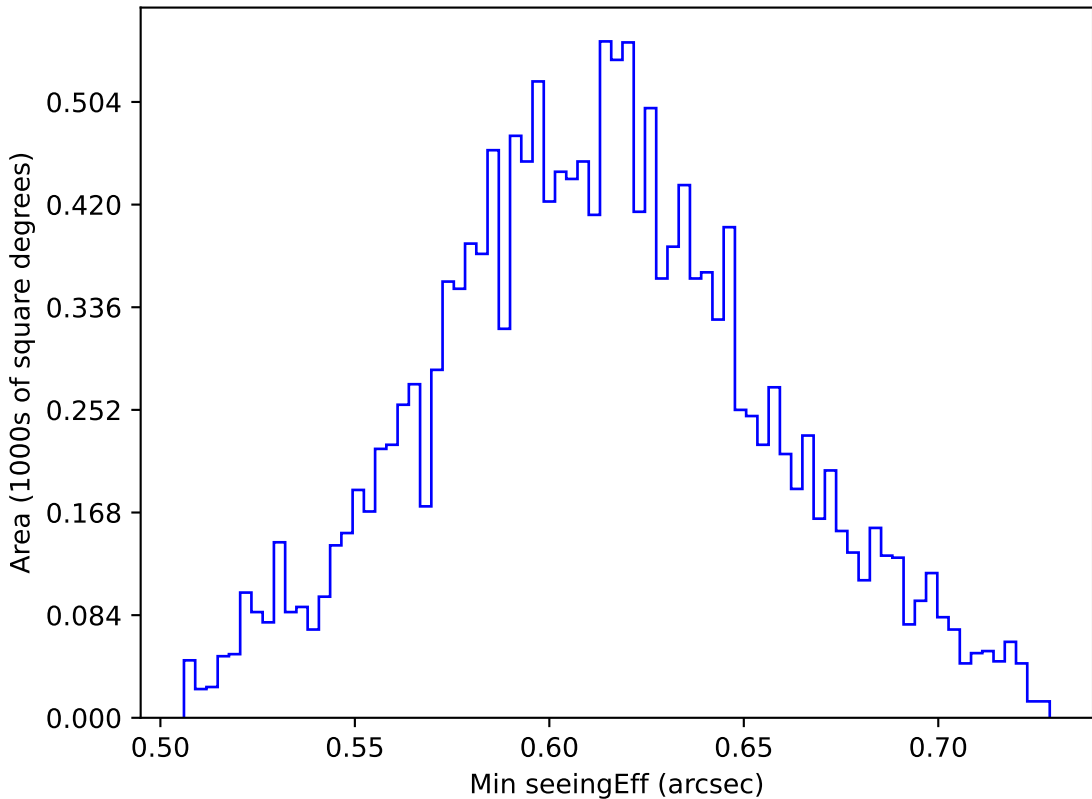
too_elab_r256_d3_ugrizy_v3.4_10yrs WFD z band: Min seeingEff
