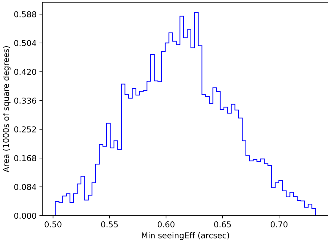
too_elab_r256_d3_ugrizy_v3.4_10yrs WFD r band: Min seeingEff
