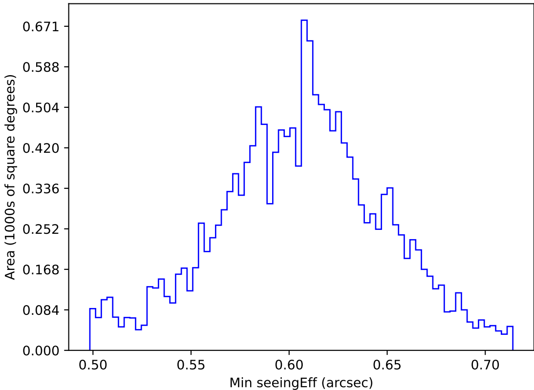
too_elab_r256_d3_ugrizy_v3.4_10yrs WFD i band: Min seeingEff
