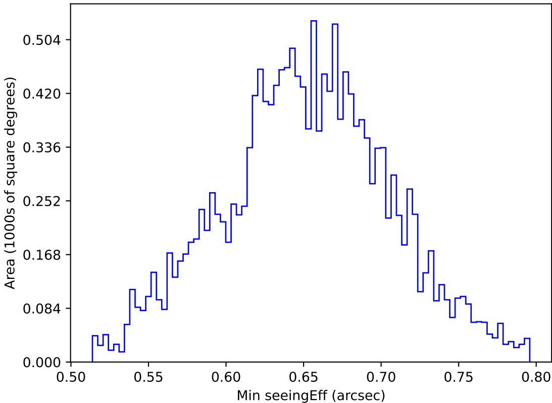
too_elab_r256_d3_ugrizy_v3.4_10yrs WFD g band: Min seeingEff
