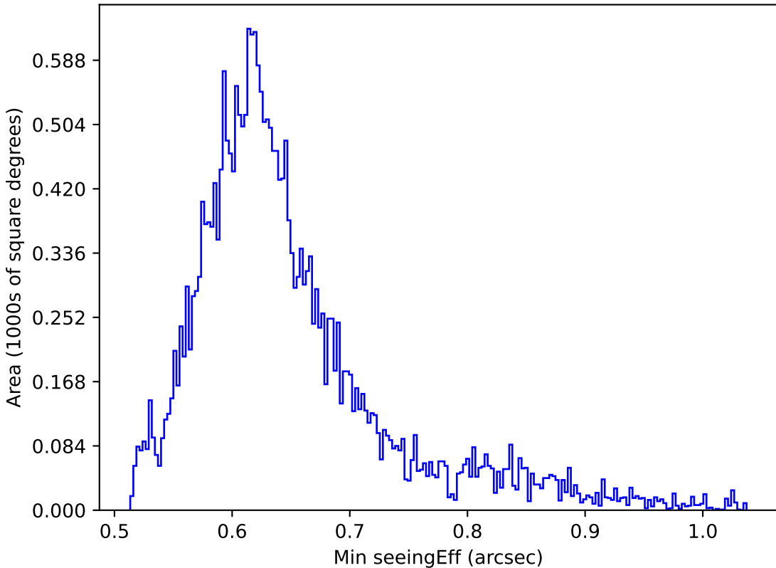
too_elab_r256_d3_ugrizy_v3.4_10yrs All sky z band: Min seeingEff
