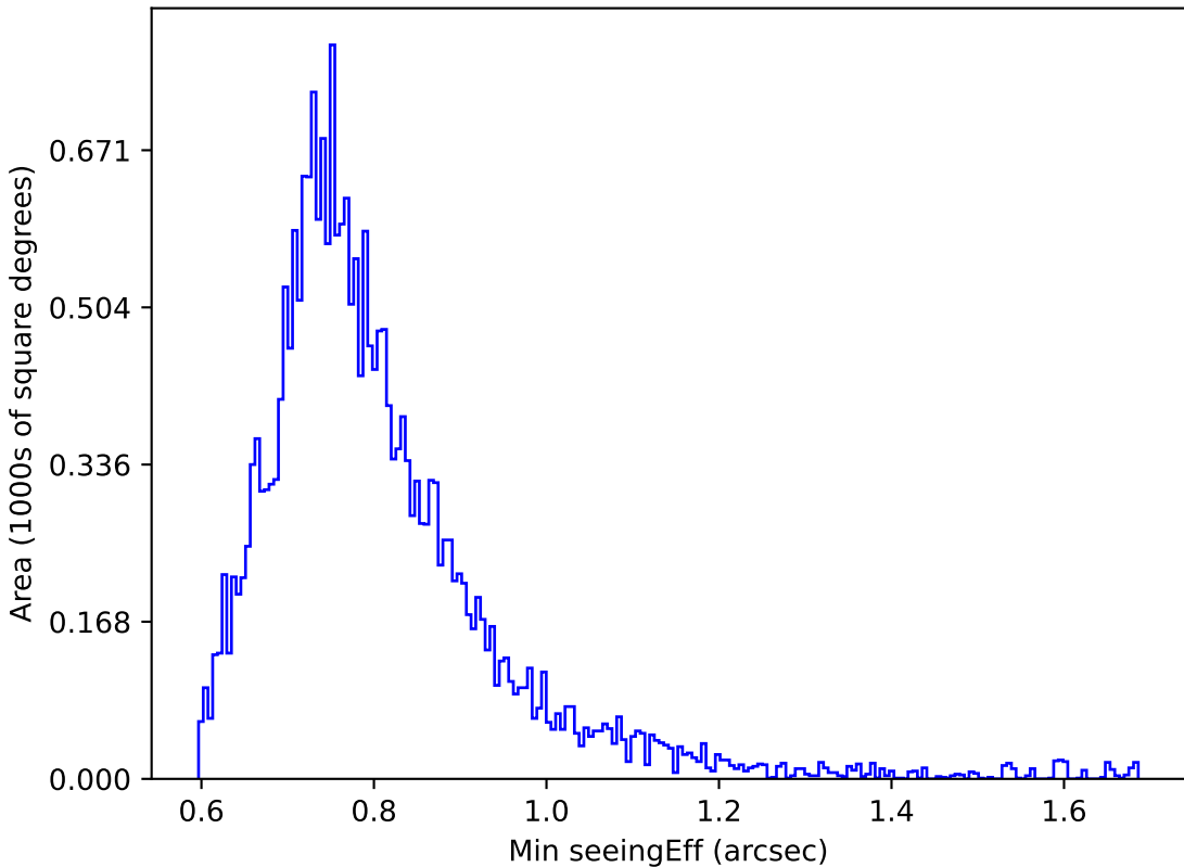
too_elab_r256_d3_ugrizy_v3.4_10yrs All sky u band: Min seeingEff
