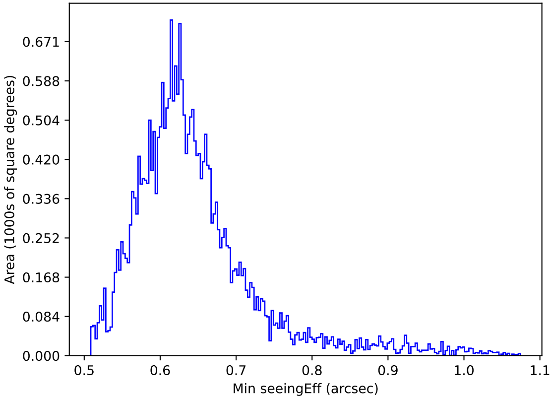
too_elab_r256_d3_ugrizy_v3.4_10yrs All sky r band: Min seeingEff
