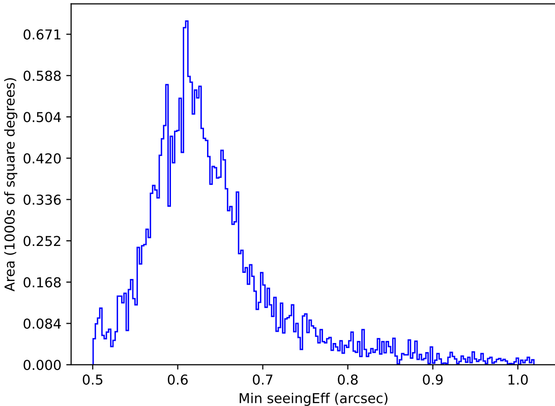
too_elab_r256_d3_ugrizy_v3.4_10yrs All sky i band: Min seeingEff
