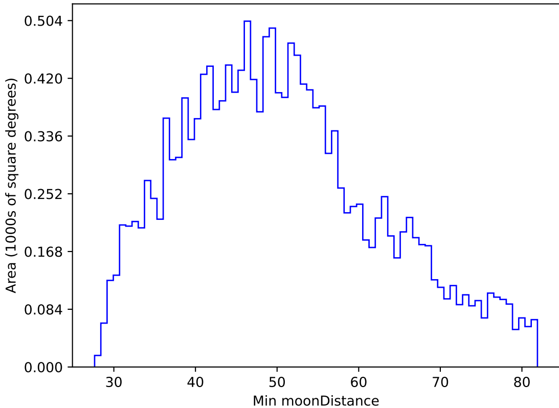
too_elab_r256_d3_ugrizy_v3.4_10yrs WFD u band: Min moonDistance
