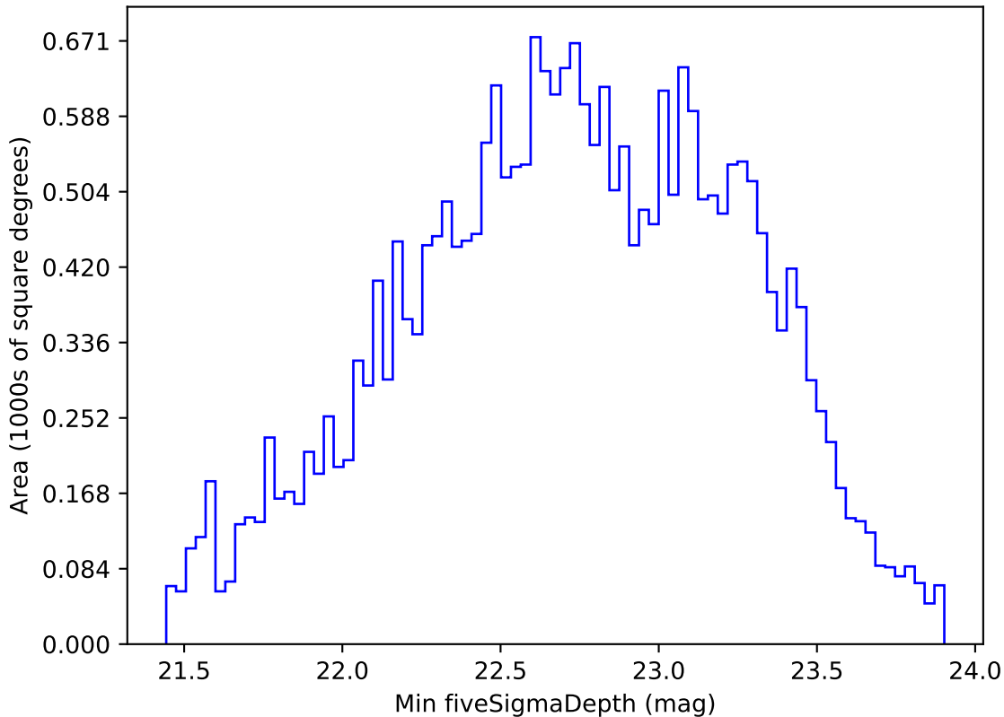
too_elab_r256_d3_ugrizy_v3.4_10yrs All sky g band: Min fiveSigmaDepth
