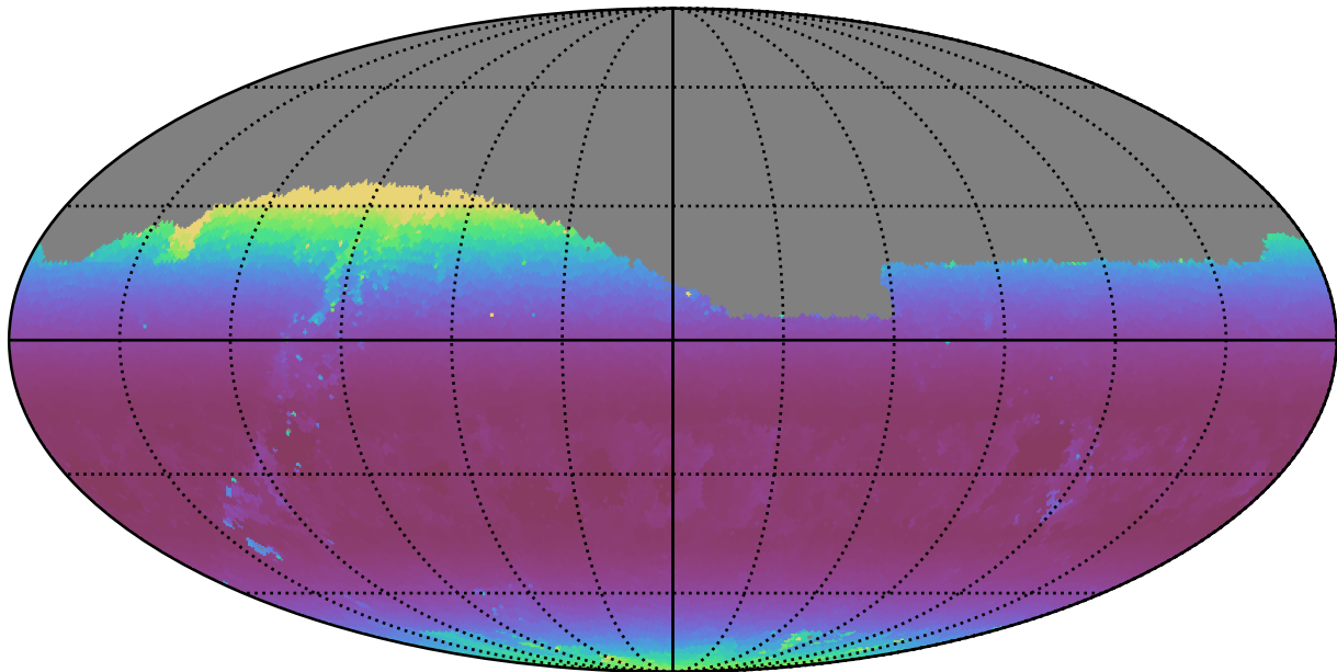
too_elab_r256_d3_ugrizy_v3.4_10yrs Yr 1 z band: Min airmass
