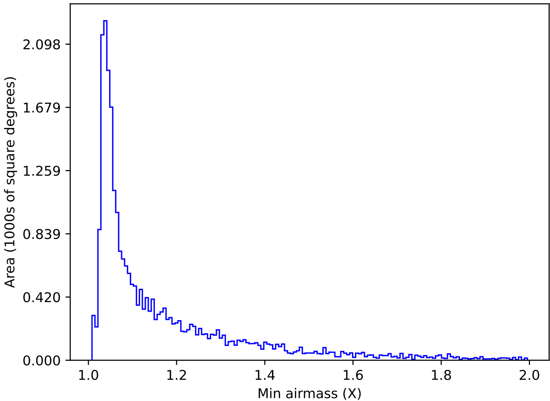
too_elab_r256_d3_ugrizy_v3.4_10yrs Yr 1 z band: Min airmass
