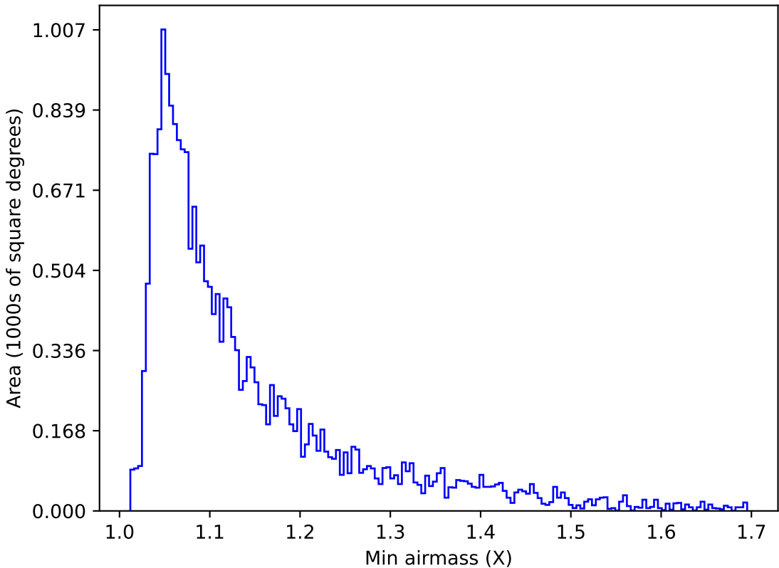
too_elab_r256_d3_ugrizy_v3.4_10yrs Yr 1 u band: Min airmass
