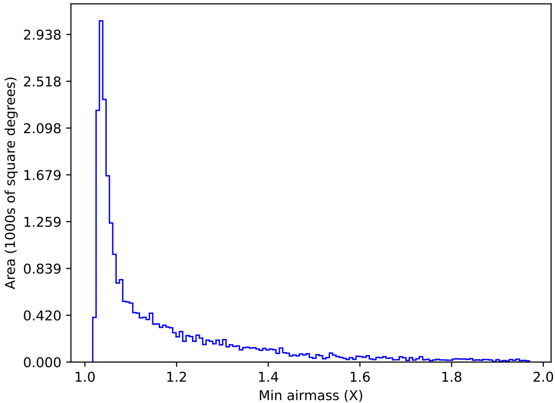
too_elab_r256_d3_ugrizy_v3.4_10yrs Yr 1 i band: Min airmass
