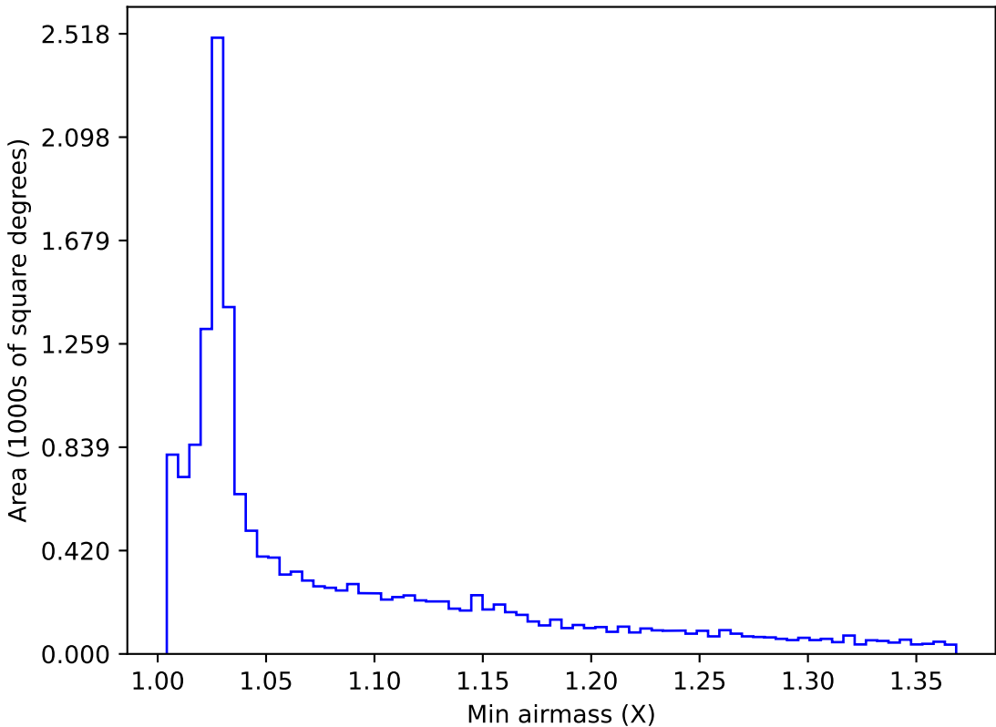
too_elab_r256_d3_ugrizy_v3.4_10yrs WFD z band: Min airmass
