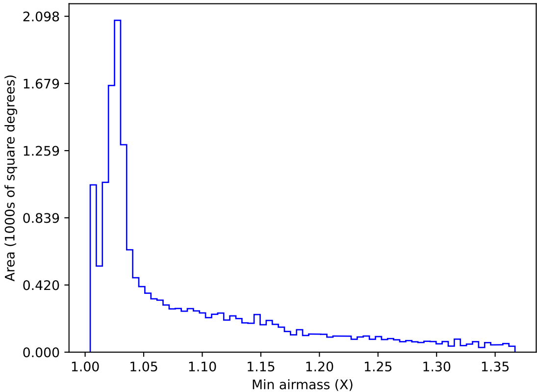
too_elab_r256_d3_ugrizy_v3.4_10yrs WFD r band: Min airmass
