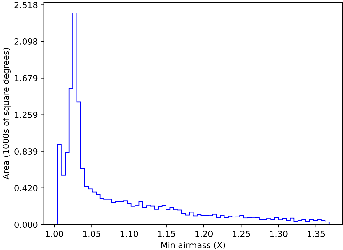
too_elab_r256_d3_ugrizy_v3.4_10yrs WFD i band: Min airmass
