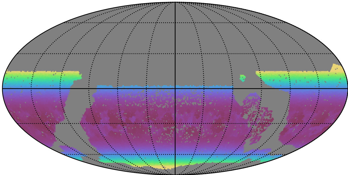
too_elab_r256_d3_ugrizy_v3.4_10yrs WFD g band: Min airmass
