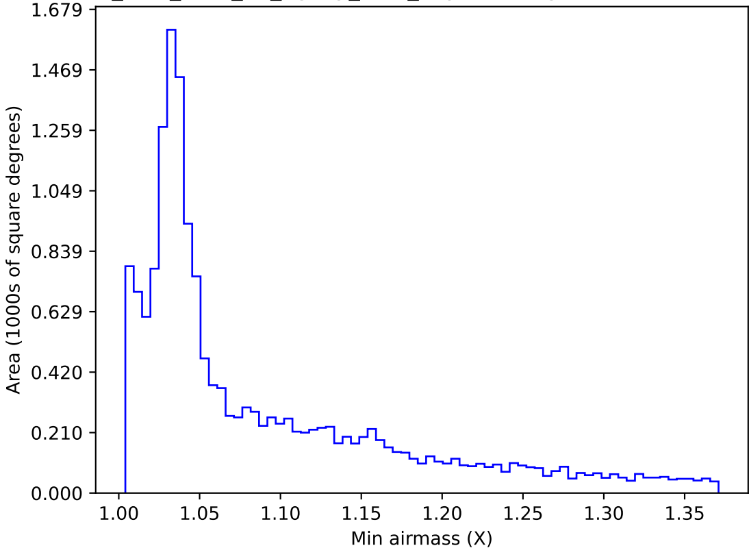
too_elab_r256_d3_ugrizy_v3.4_10yrs WFD g band: Min airmass
