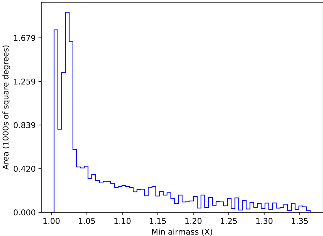
too_elab_r256_d3_ugrizy_v3.4_10yrs WFD all bands: Min airmass
