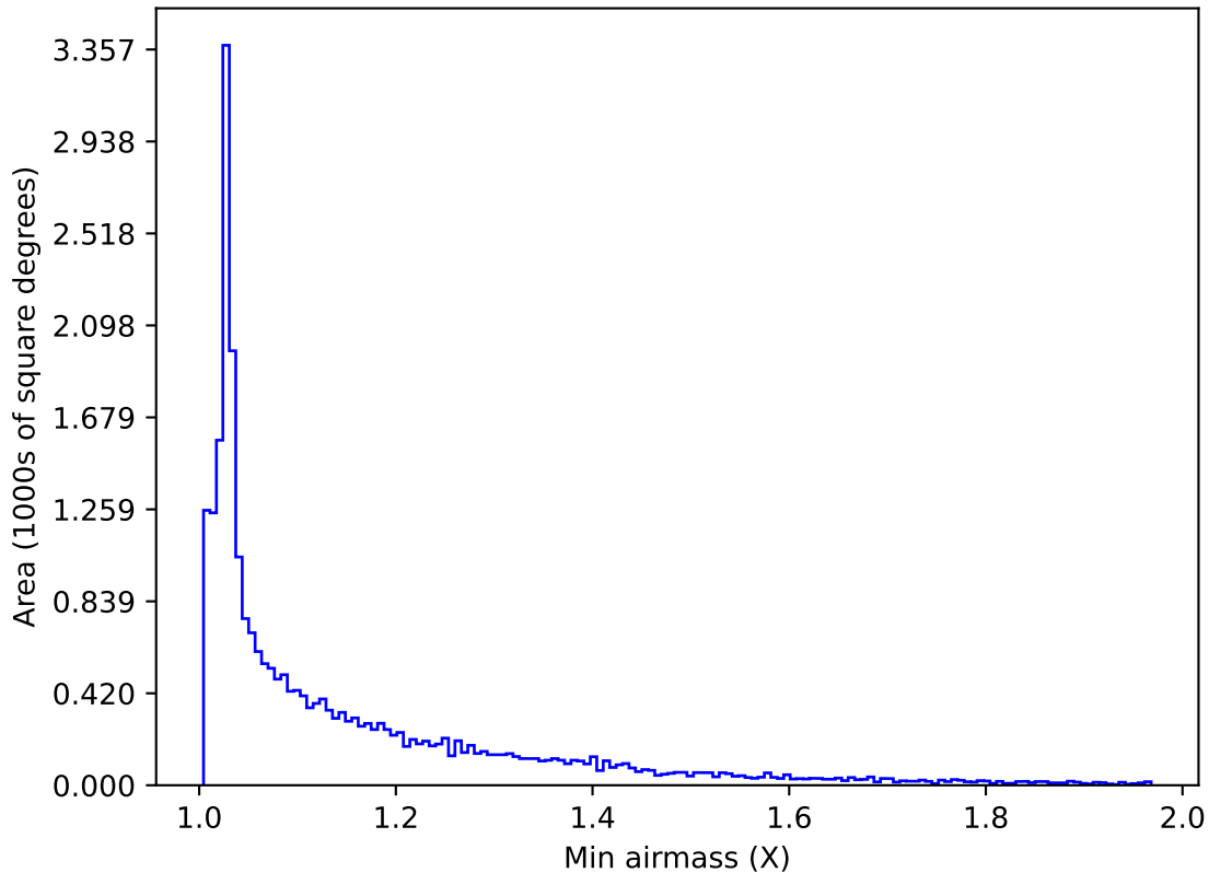
too_elab_r256_d3_ugrizy_v3.4_10yrs All sky z band: Min airmass
