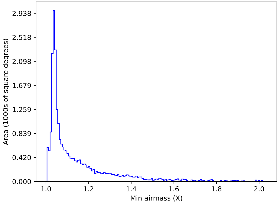
too_elab_r256_d3_ugrizy_v3.4_10yrs All sky u band: Min airmass
