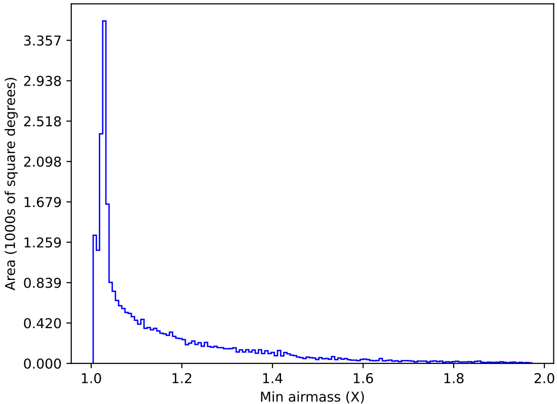
too_elab_r256_d3_ugrizy_v3.4_10yrs All sky i band: Min airmass
