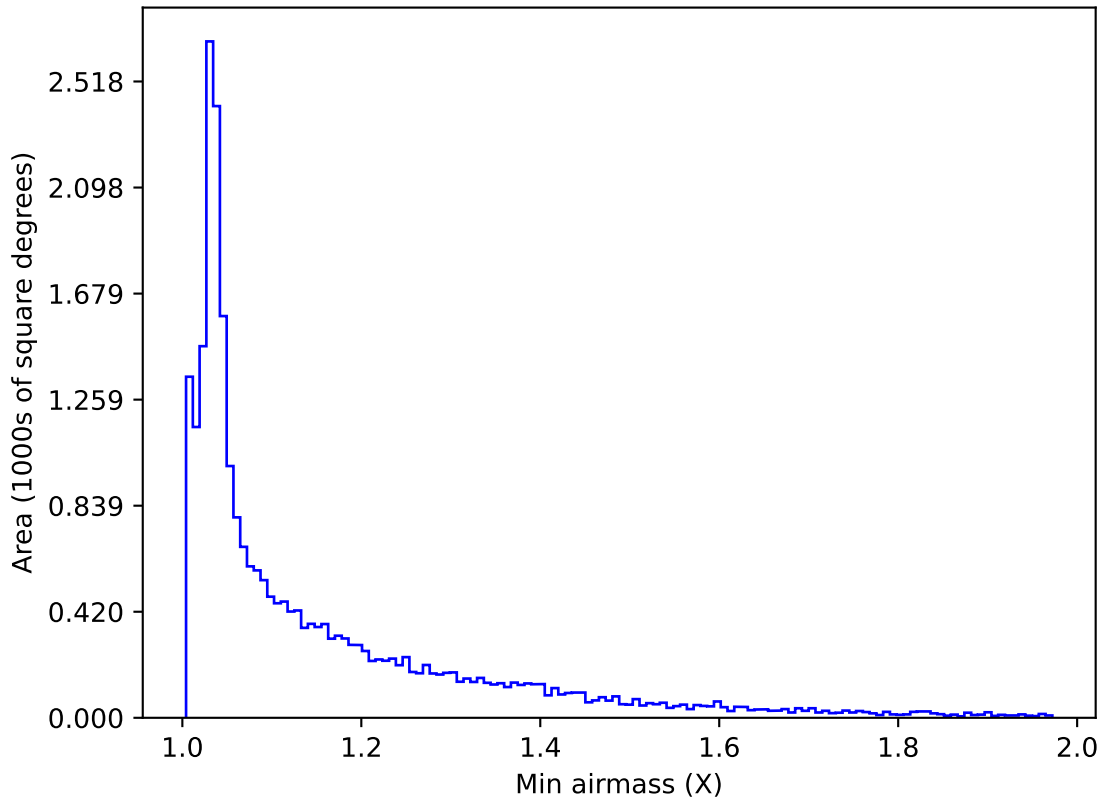
too_elab_r256_d3_ugrizy_v3.4_10yrs All sky g band: Min airmass
