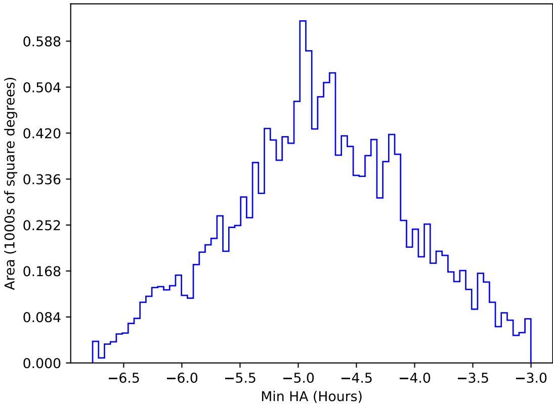
too_elab_r256_d3_ugrizy_v3.4_10yrs WFD all bands: Min HA
