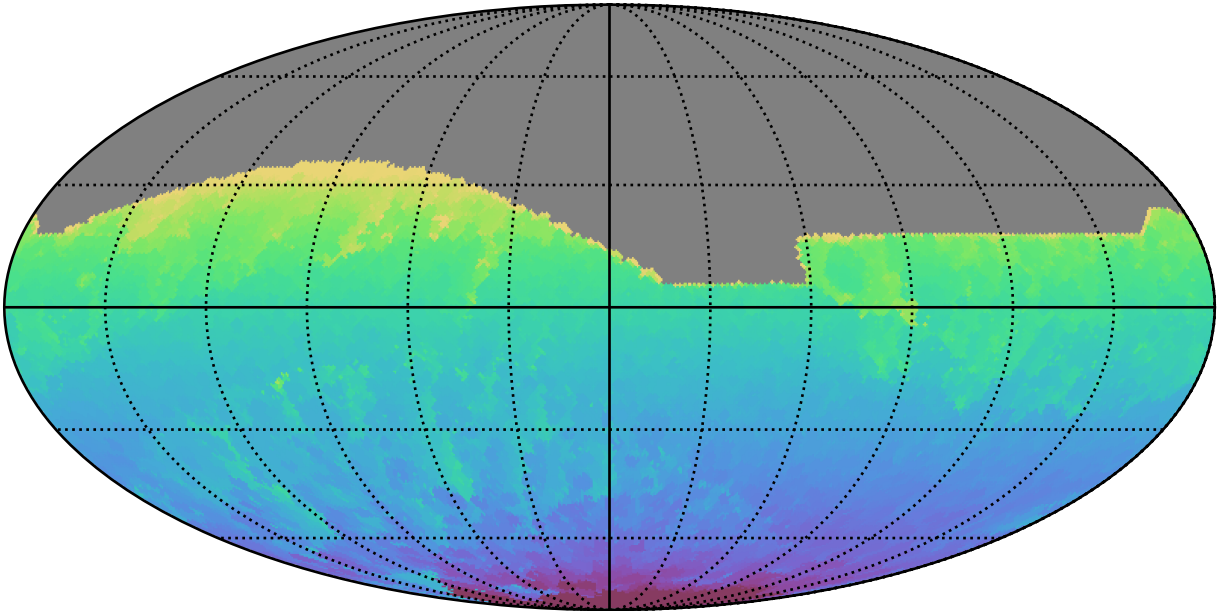
too_elab_r256_d3_ugrizy_v3.4_10yrs All sky all bands: Min HA
