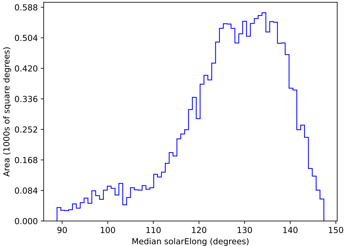
too_elab_r256_d3_ugrizy_v3.4_10yrs WFD z band: Median solarElong
