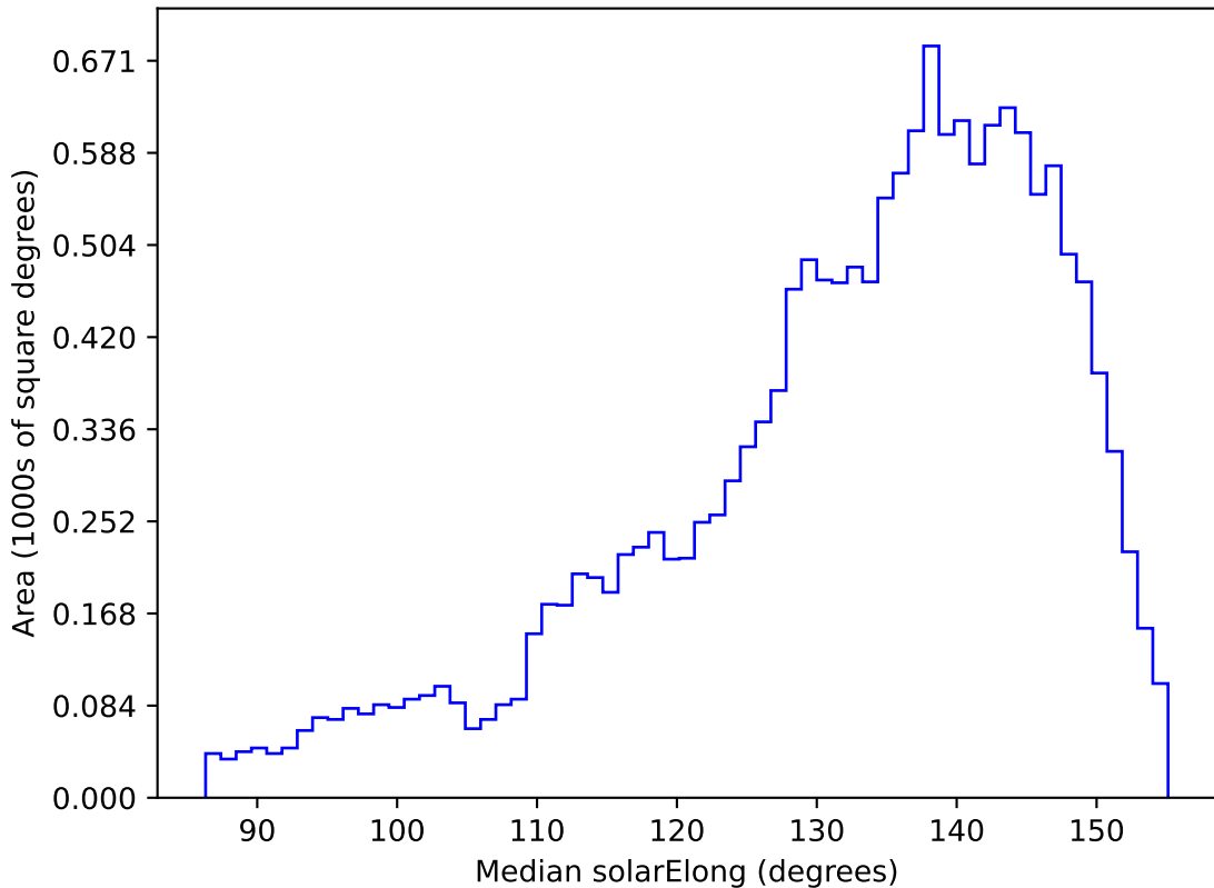
too_elab_r256_d3_ugrizy_v3.4_10yrs WFD u band: Median solarElong
