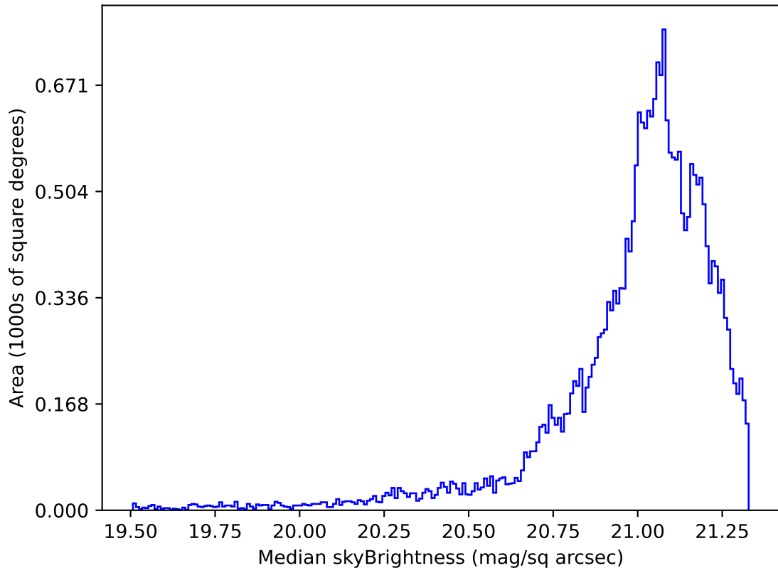
too_elab_r256_d3_ugrizy_v3.4_10yrs Yr 1 r band: Median skyBrightness
