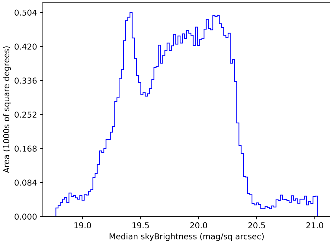
too_elab_r256_d3_ugrizy_v3.4_10yrs Yr 1 all bands: Median skyBrightness
