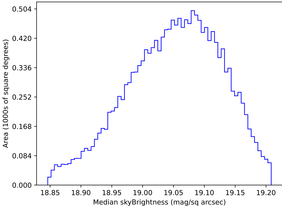
too_elab_r256_d3_ugrizy_v3.4_10yrs WFD z band: Median skyBrightness
