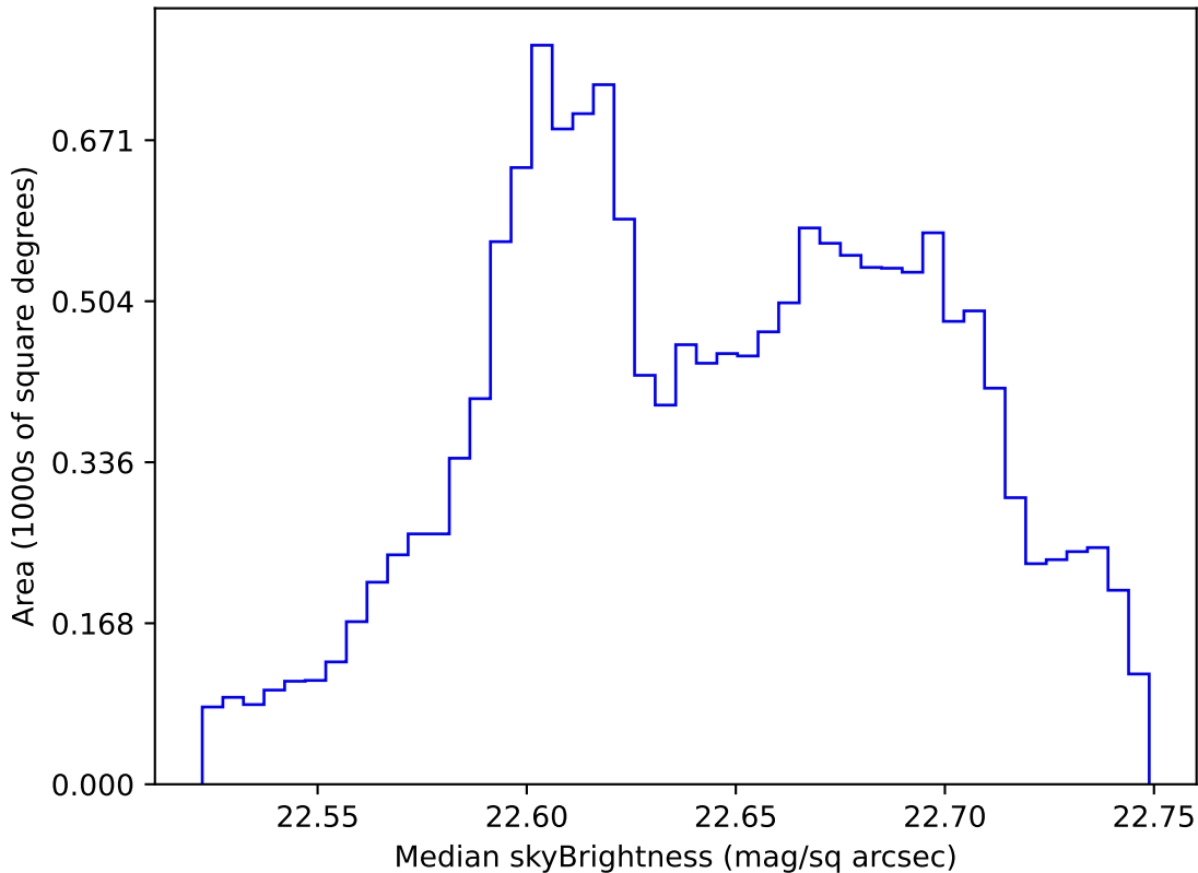
too_elab_r256_d3_ugrizy_v3.4_10yrs WFD u band: Median skyBrightness
