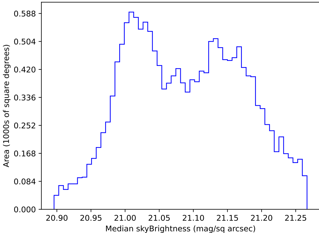
too_elab_r256_d3_ugrizy_v3.4_10yrs WFD r band: Median skyBrightness
