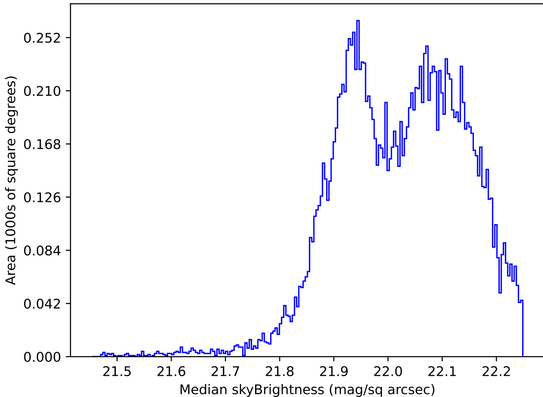
too_elab_r256_d3_ugrizy_v3.4_10yrs WFD g band: Median skyBrightness
