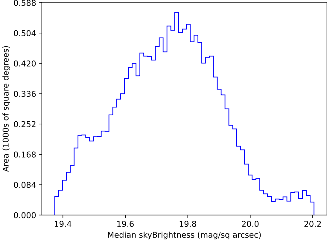
too_elab_r256_d3_ugrizy_v3.4_10yrs WFD all bands: Median skyBrightness
