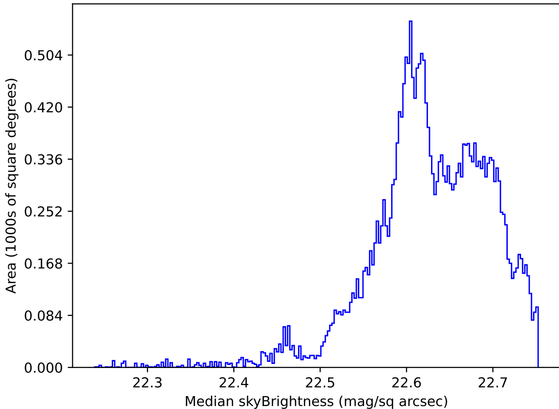
too_elab_r256_d3_ugrizy_v3.4_10yrs All sky u band: Median skyBrightness
