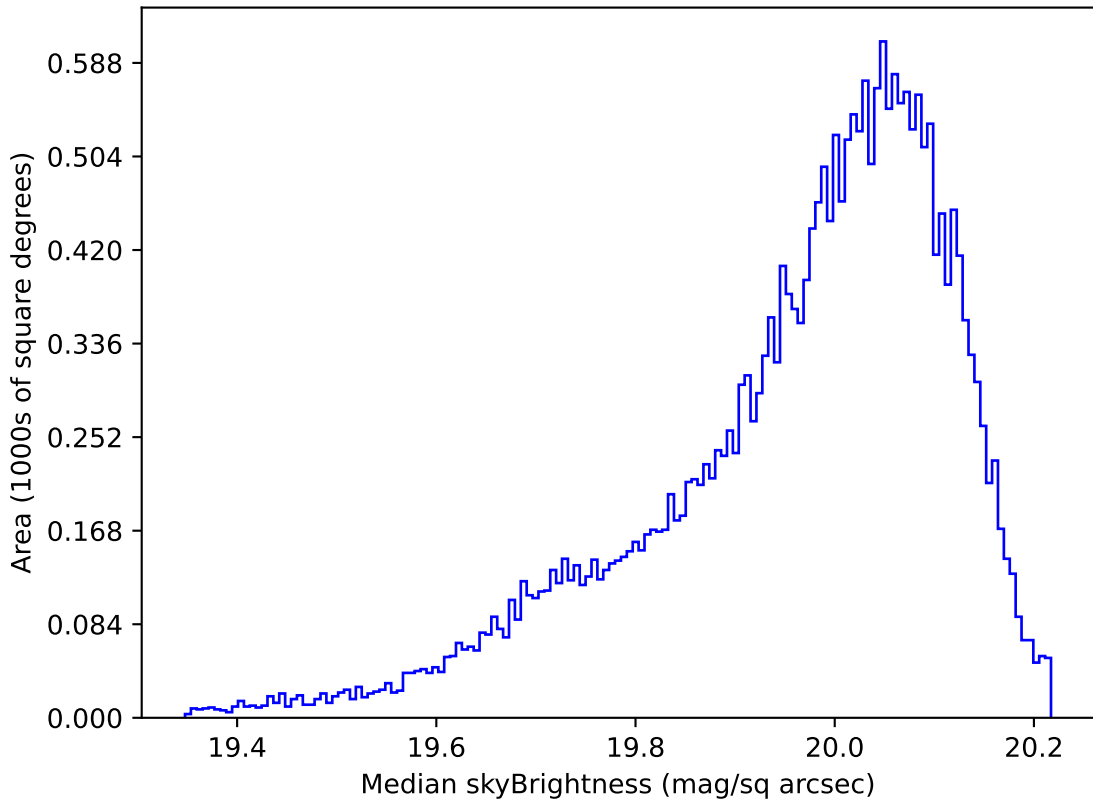
too_elab_r256_d3_ugrizy_v3.4_10yrs All sky i band: Median skyBrightness
