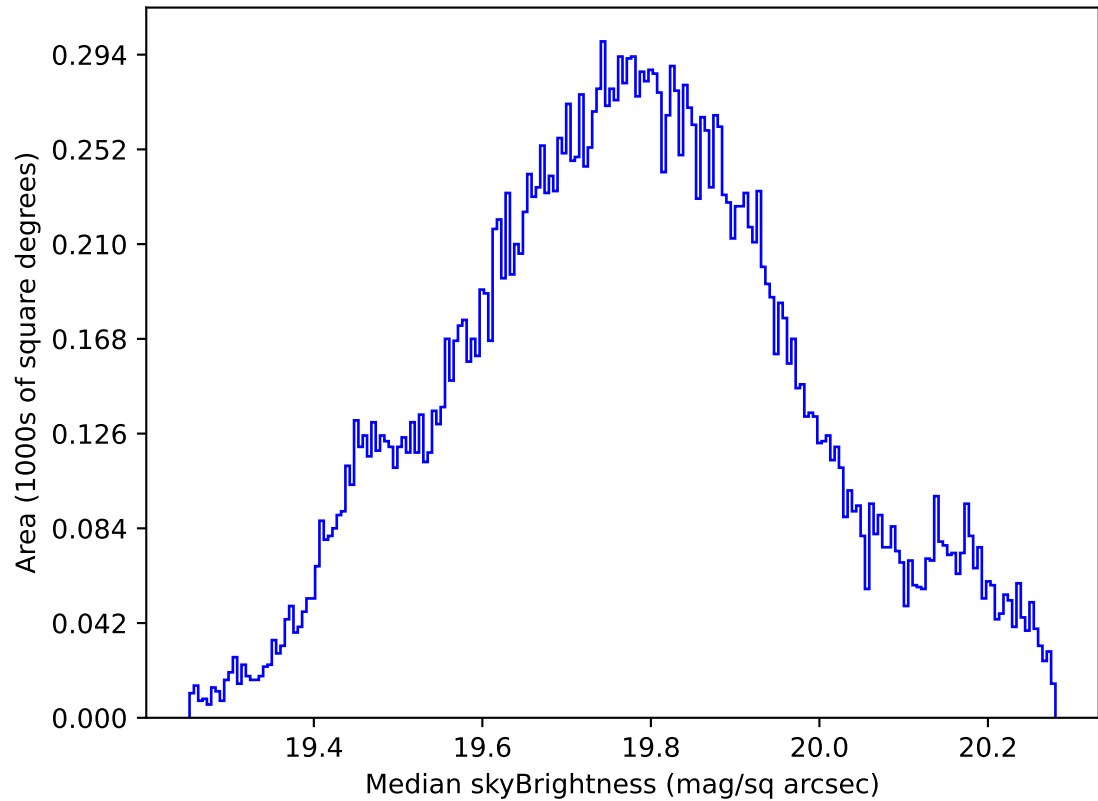
too_elab_r256_d3_ugrizy_v3.4_10yrs All sky all bands: Median skyBrightness
