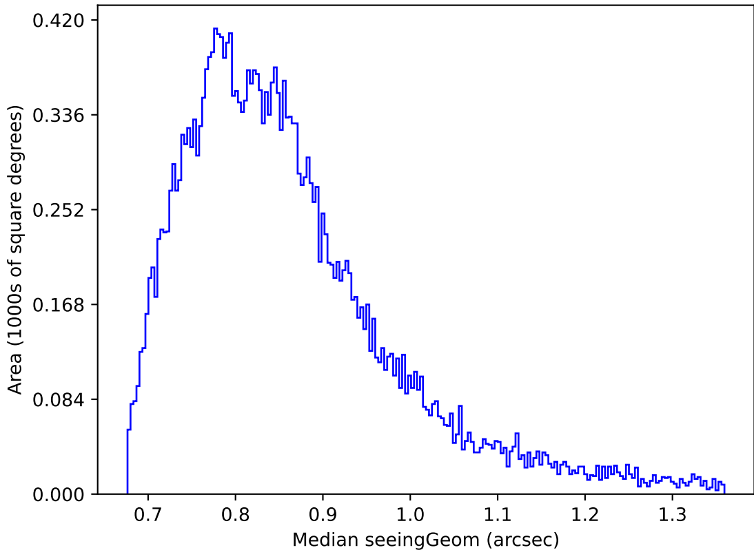
too_elab_r256_d3_ugrizy_v3.4_10yrs Yr 1 r band: Median seeingGeom
