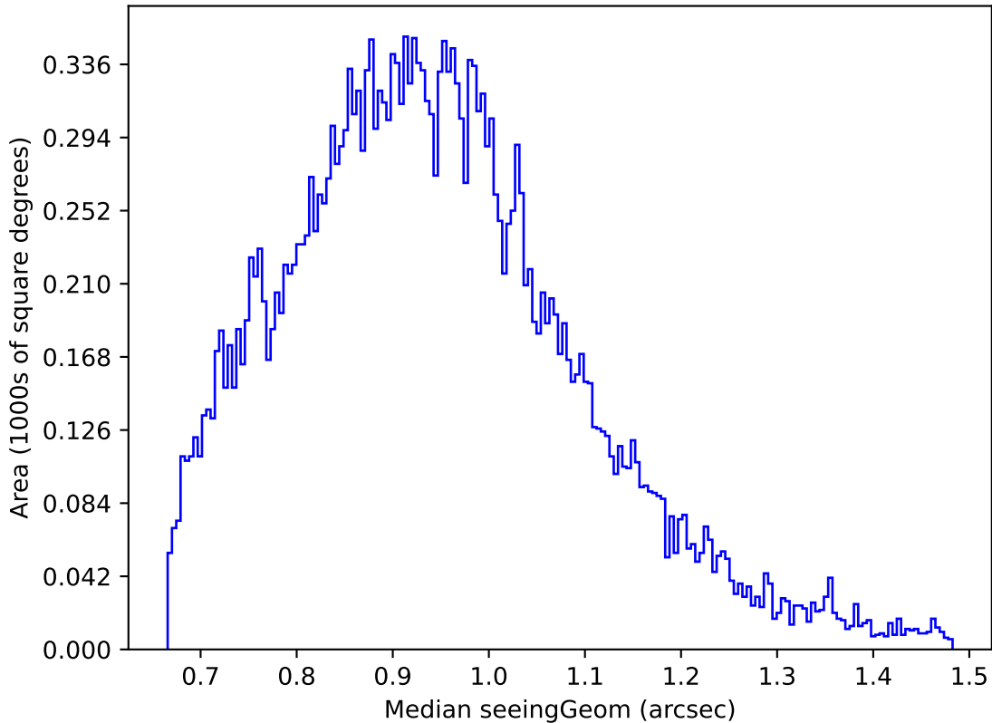
too_elab_r256_d3_ugrizy_v3.4_10yrs Yr 1 g band: Median seeingGeom
