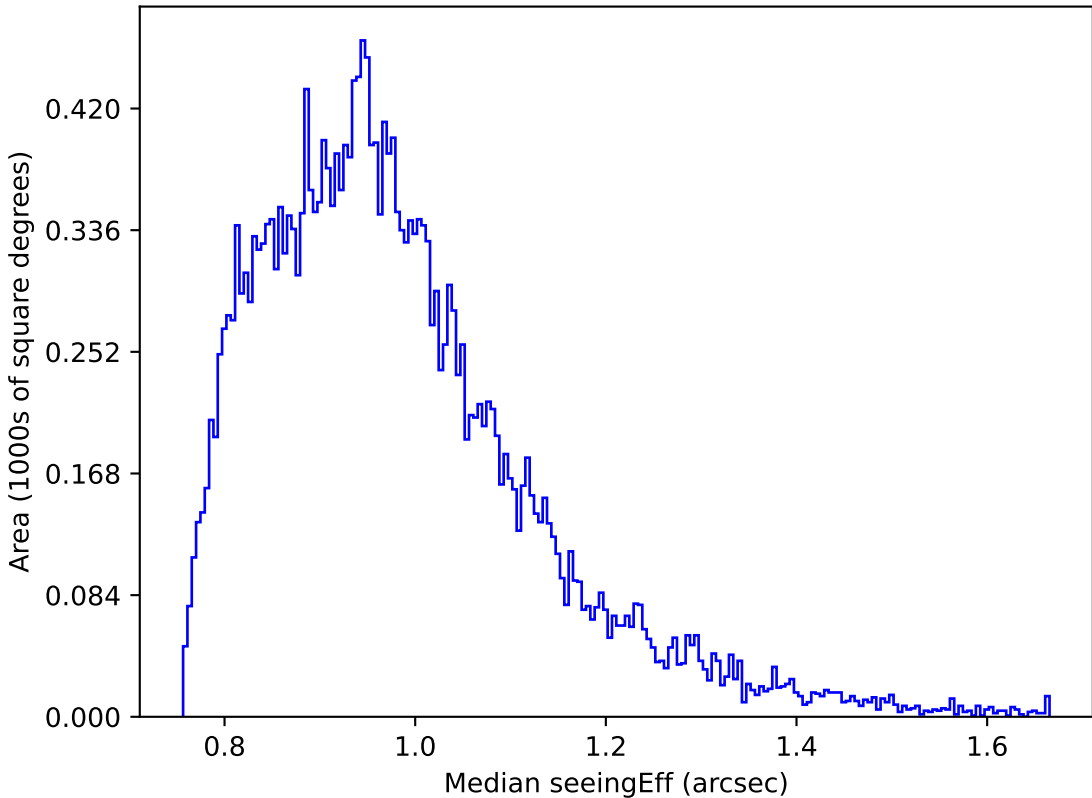
too_elab_r256_d3_ugrizy_v3.4_10yrs Yr 1 z band: Median seeingEff
