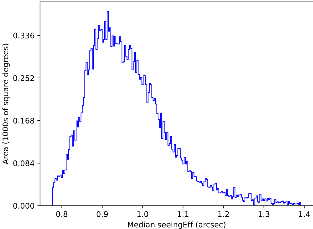
too_elab_r256_d3_ugrizy_v3.4_10yrs Yr 1 y band: Median seeingEff
