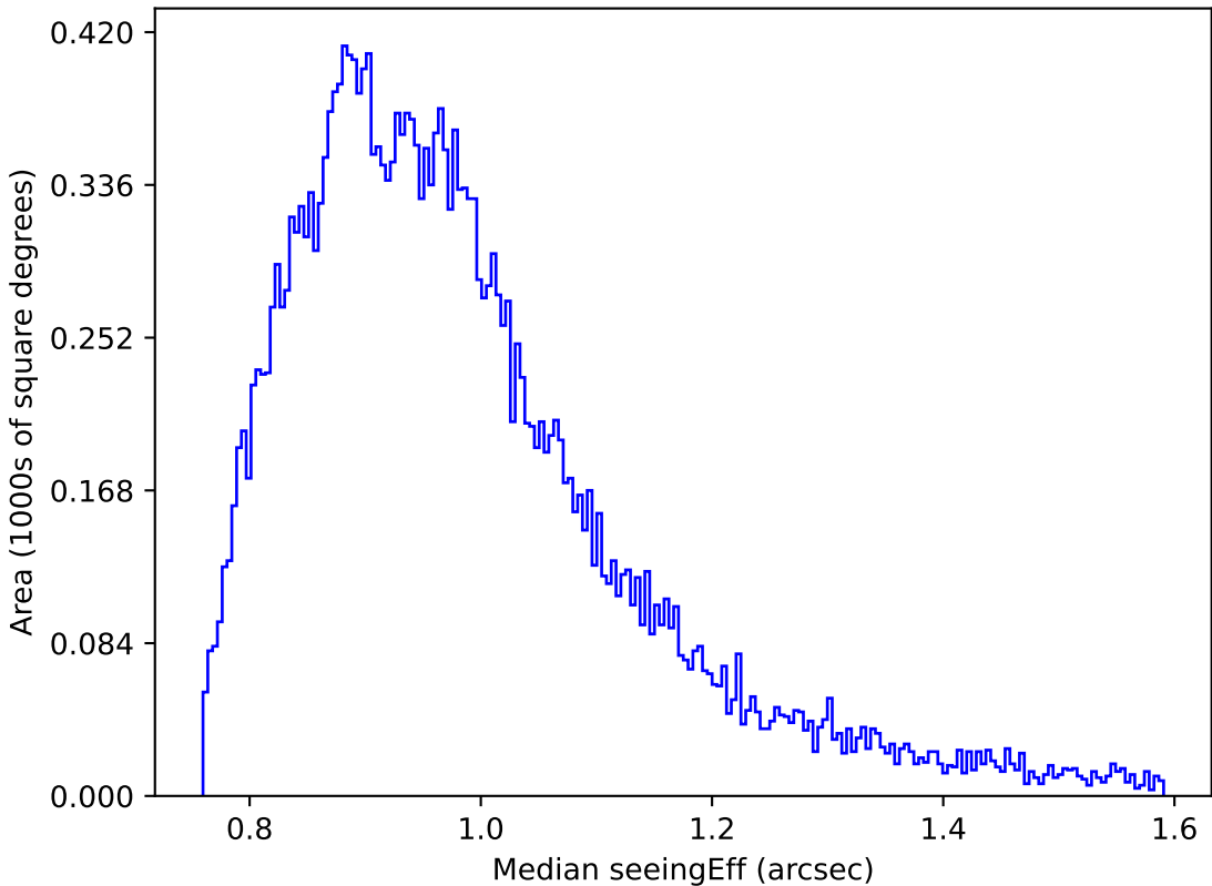
too_elab_r256_d3_ugrizy_v3.4_10yrs Yr 1 r band: Median seeingEff
