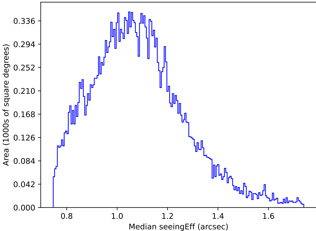
too_elab_r256_d3_ugrizy_v3.4_10yrs Yr 1 g band: Median seeingEff
