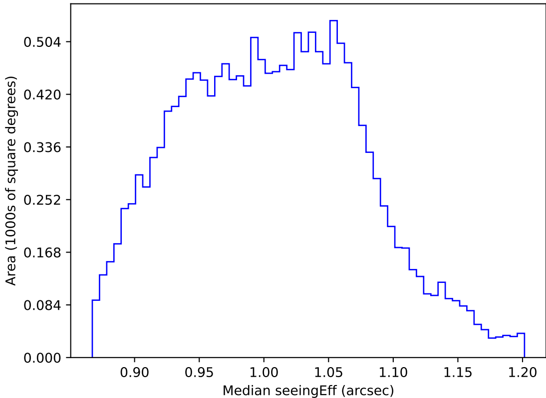
too_elab_r256_d3_ugrizy_v3.4_10yrs WFD z band: Median seeingEff
