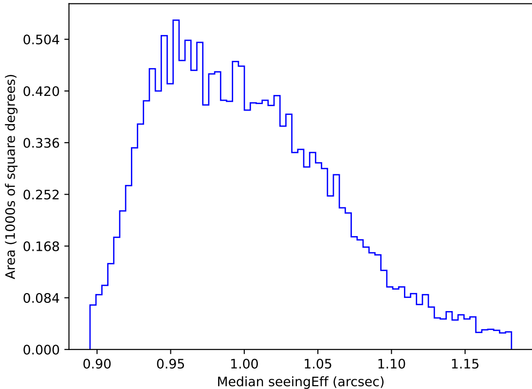
too_elab_r256_d3_ugrizy_v3.4_10yrs WFD y band: Median seeingEff
