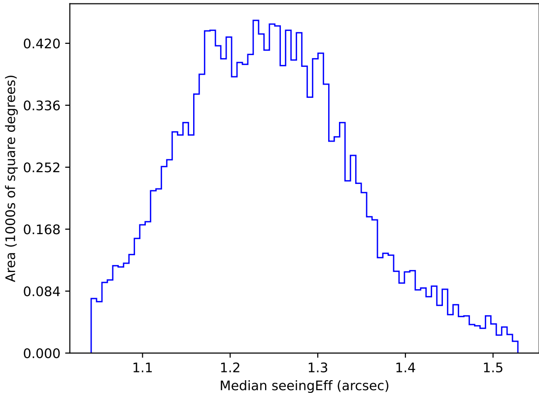
too_elab_r256_d3_ugrizy_v3.4_10yrs WFD u band: Median seeingEff
