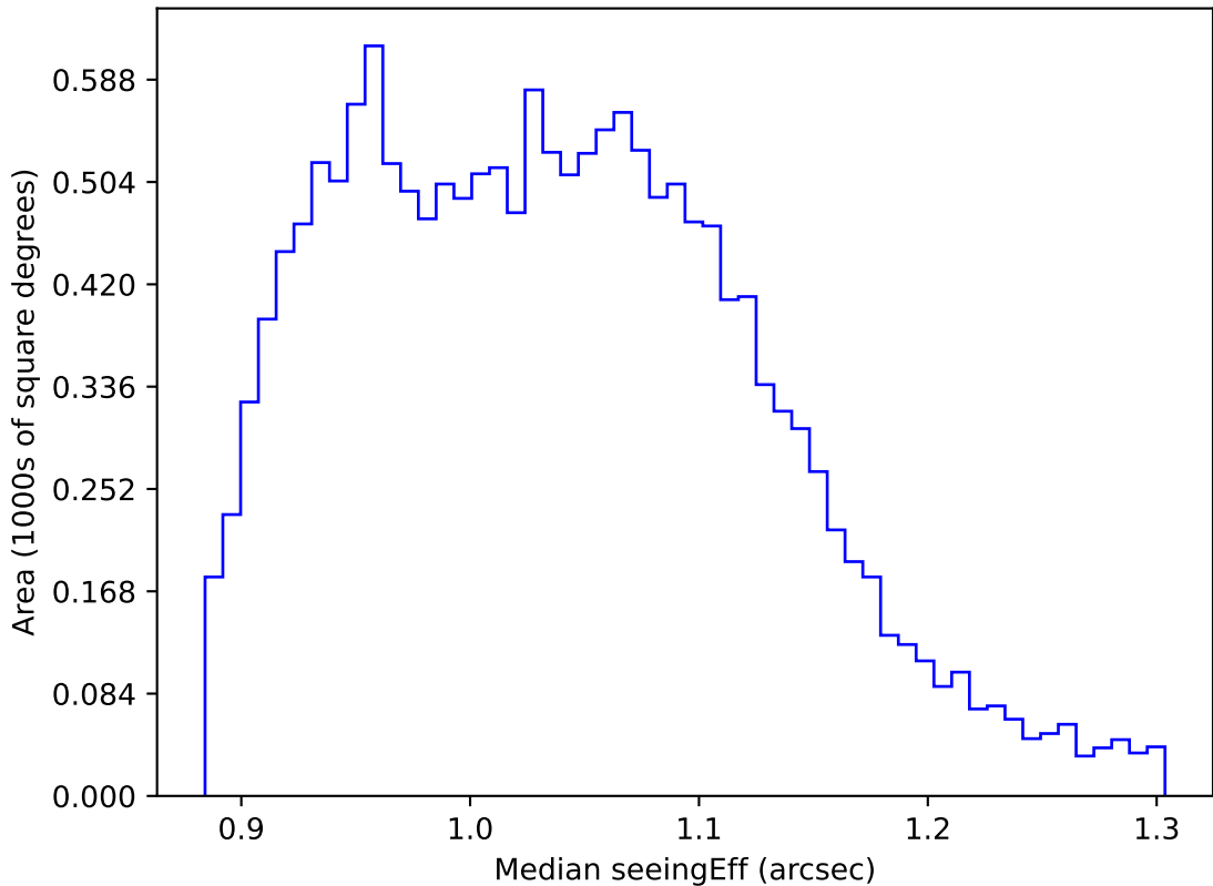
too_elab_r256_d3_ugrizy_v3.4_10yrs WFD r band: Median seeingEff
